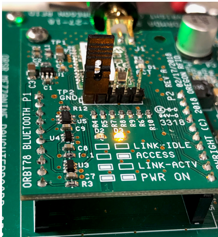
Jumper inserted between GND and next pin
